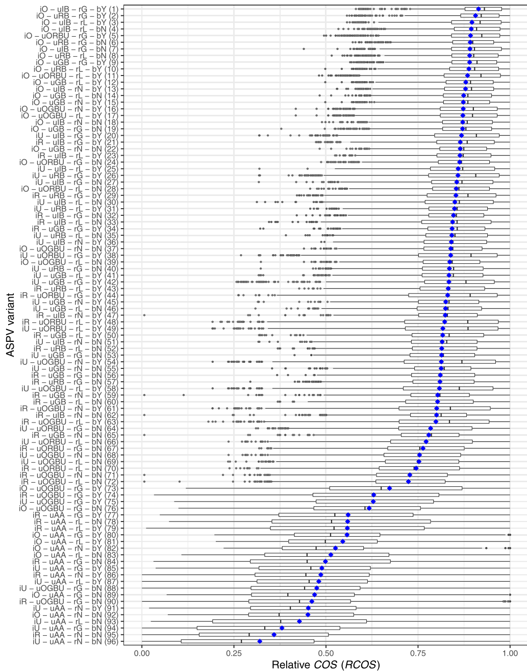
Fig. 1. Distribution of the \overline{RCOS}^{eval} values (calculated on a per instance basis) for all 30 runs of each ASPV variant on all instances; blue diamonds represent the per variant average \overline{RCOS}^{eval}(v) (M-Eval phase). (For interpretation of the references to color in this figure legend, the reader is referred to the web version of this article.)
